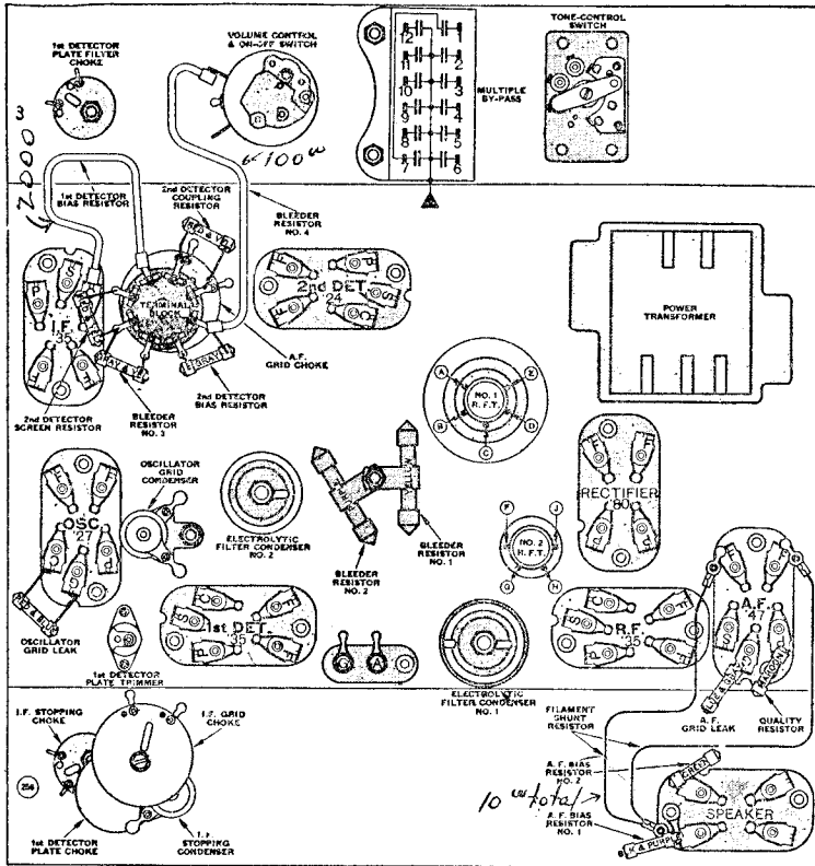
BOTTOM CHART.
